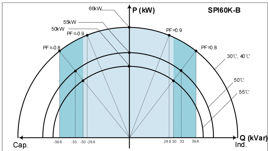
P-Q curve at 1.1/1.05/1 U_n @30°C,40°C,50°C,55°C
