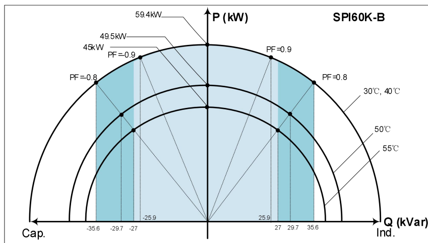
P-Q curve at 0.90 U_n @30°C,40°C,50°C,55°C
