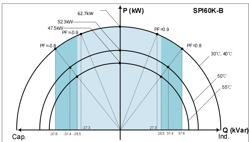
P-Q curve at 0.95 U_n @30°C,40°C,50°C,55°C
