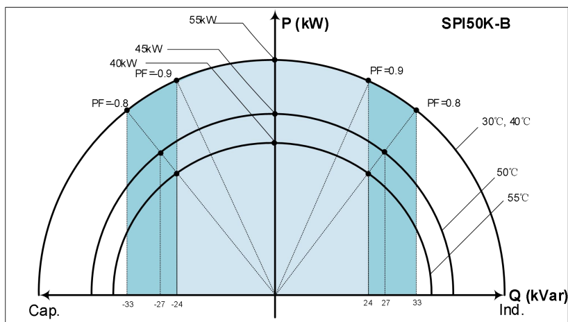
P-Q curve at 1.1/1.05/1 Un @30°C,40°C,50°C,55°C
